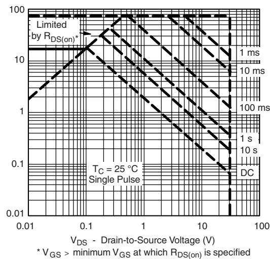
Safe Operating Area, Junction-to-Case
