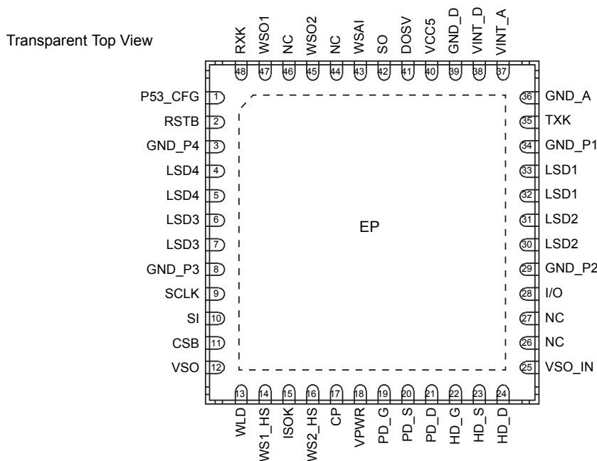
Figure 3. SB0400 48-pin QFN-EP pinout diagram
