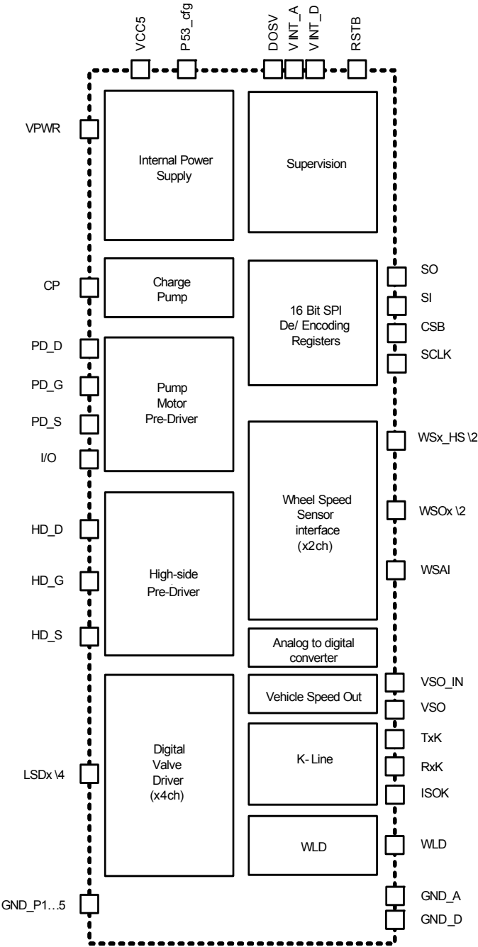
Figure 2. SB0400 simplified block diagram
