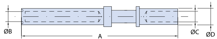
Socket Crimp Contact Part Numbers, Size & Dimensions Table 2/2
