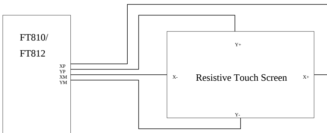
Figure 4-8 Resistive Touch screen connection
