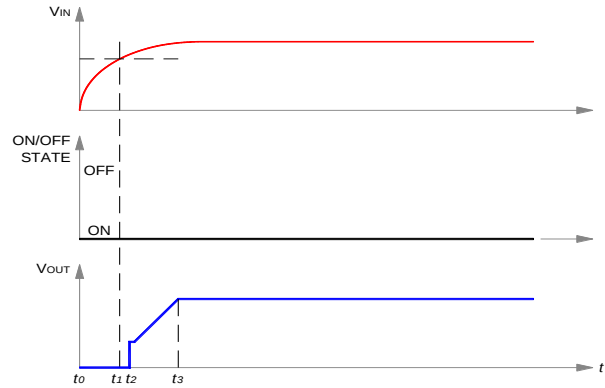
Figure 6. Start-up scenario #1.
