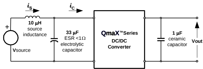
Figure 21. Test setup for measuring input reflected ripple currents, i_c and i_s .
