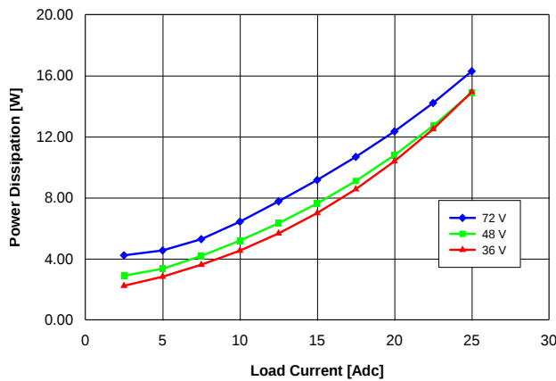
Figure 15. Power dissipation vs. load current and input voltage for converter mounted vertically with air flowing from pin 3 to pin 1 at a rate of 300 LFM (1.5 m/s) and T_a = 25^\circ\text{C} .
