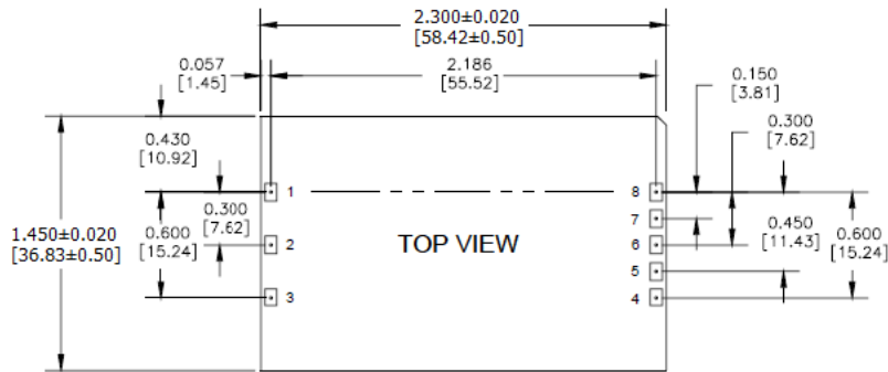
QMS48 (SurfaceMount)
