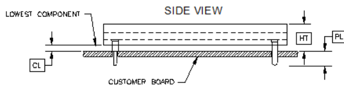
QM48T (Through-Hole)
