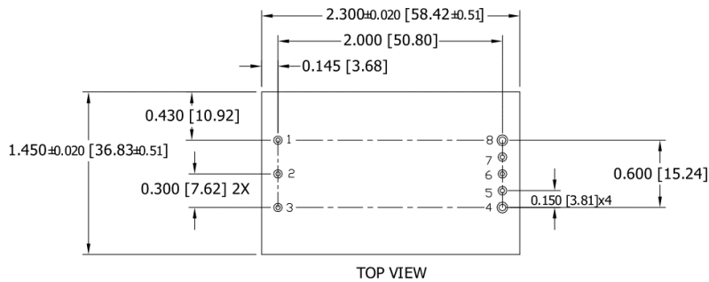
QM48T (Through-Hole)
