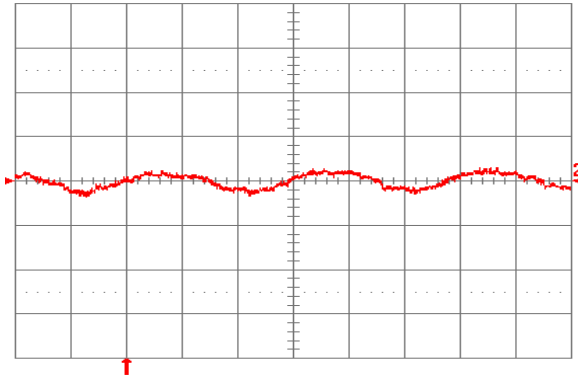
Figure 22. Input reflected ripple current, i_s (10 mA/div), measured through 10 \mu H at the source at full rated load current and V_{in} = 48 V. Refer to Fig. 21 for test setup. Time scale: 1 \mu s/div.
