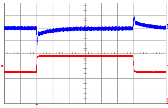
Figure 19. Output voltage response to load current step-change (12.5 A – 18.75 A – 12.5 A) at V_{in} = 48\text{ V} . Top trace: output voltage (100 mV/div.). Bottom trace: load current (5 A/div.). Current slew rate: 1 A/ \mu\text{s} . C_o = 470\text{ }\mu\text{F} tantalum + 1 \mu\text{F} ceramic. Time scale: 0.2 ms/div.
