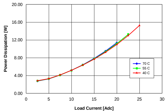
Figure 16. Power dissipation vs. load current and ambient temperature for converter mounted vertically with V_{in} = 48\text{ V} and air flowing from pin 3 to pin 1 at a rate of 200 LFM (1.0 m/s).
