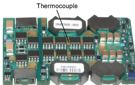
Figure 5. Location of the thermocouple for thermal testing
