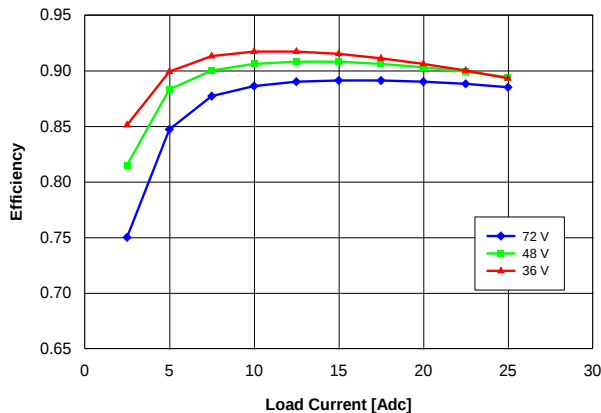
Figure 13. Efficiency vs. load current and input voltage for converter mounted vertically with air flowing from pin 3 to pin 1 at a rate of 300 LFM (1.5 m/s) and T_a = 25^{\circ}\text{C} .
