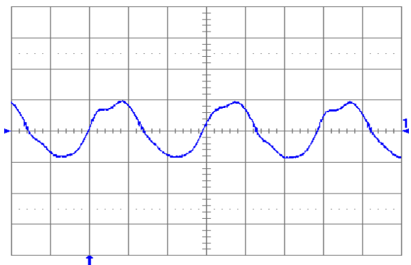
Figure 20. Output voltage ripple (20 mV/div.) at full rated load current into a resistive load with C_o = 10\text{ }\mu\text{F} tantalum + 1 \mu\text{F} ceramic and V_{in} = 48\text{ V} . Time scale: 1 \mu\text{s} /div.
