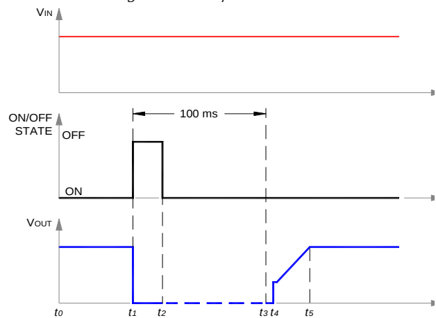
Figure 8. Startup scenario #3.
