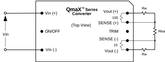
Figure 2. Remote sense circuit configuration
