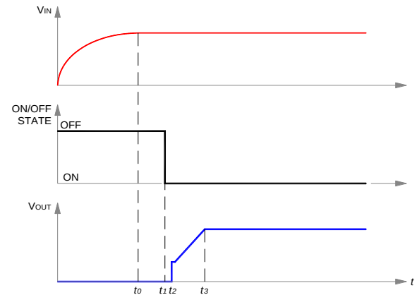
Figure 7. Startup scenario #2.
