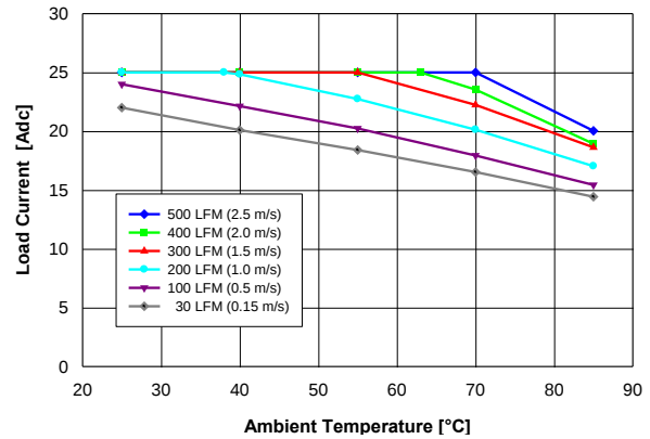
Figure 10. Available load current vs. ambient air temperature and airflow rates for QM48T25050 converter with B height pins mounted horizontally with air flowing from pin 3 to pin 1, MOSFET temperature \leq 120^{\circ}\text{C} , V_{in} = 48\text{ V} .
