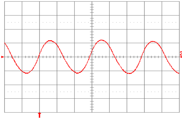
Figure 23. Input reflected ripple current, i_c (200 mA/div), measured at input terminals at full rated load current and V_{in} = 48 V. Refer to Fig. 21 for test setup. Time scale: 1 \mu s/div.
