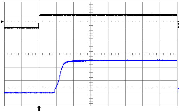
Figure 17. Turn-on transient at full rated load current (resistive) with no output capacitor at V_{in} = 48\text{ V} , triggered via ON/OFF pin. Top trace: ON/OFF signal (5 V/div.). Bottom trace: output voltage (2 V/div.). Time scale: 2 ms/div.
