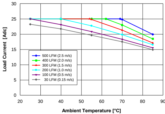
Figure 9. Available load current vs. ambient air temperature and airflow rates for QM48T25050 converter with B height pins mounted vertically with air flowing from pin 3 to pin 1, MOSFET temperature \leq 120^{\circ}\text{C} , V_{in} = 48\text{ V} .
