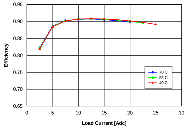
Figure 14. Efficiency vs. load current and ambient temperature for converter mounted vertically with V_{in} = 48\text{ V} and air flowing from pin 3 to pin 1 at a rate of 200 LFM (1.0 m/s).
