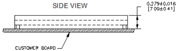
QMS48 (SurfaceMount)
