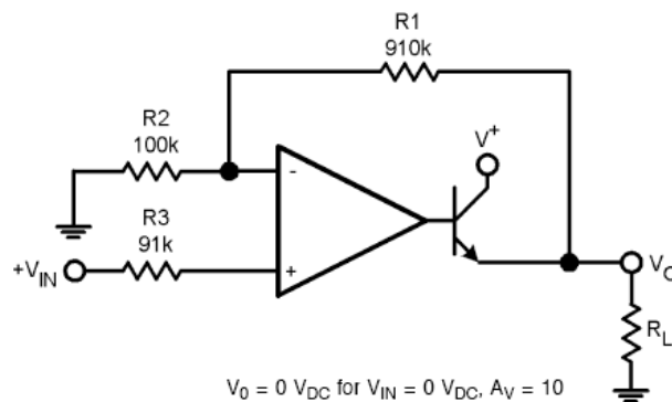
Figure 6. Power Amplifier
