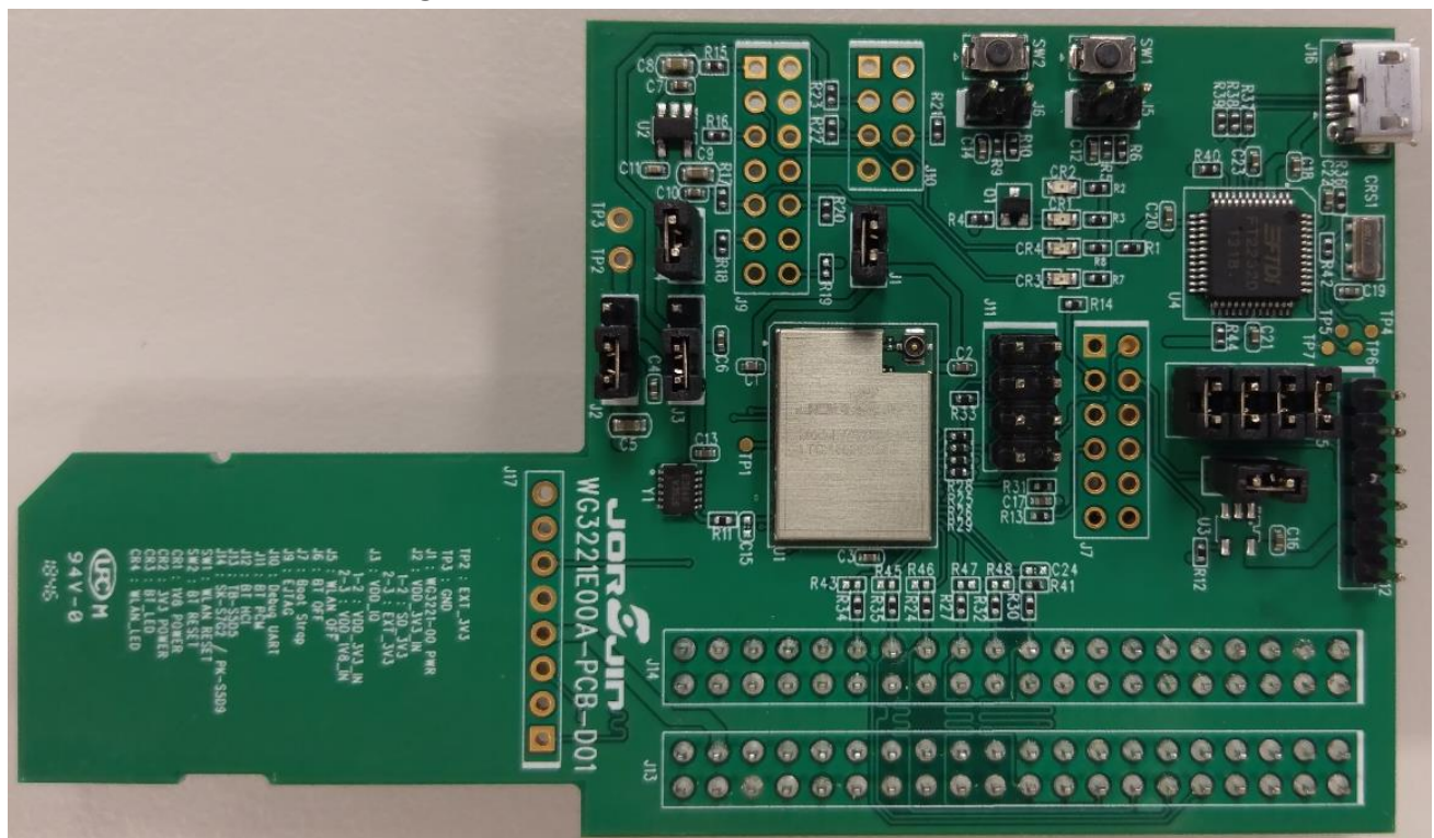
Figure 1: WG3221E00 Evaluation Board
