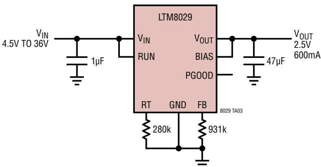
2.5V Step-Down Converter
