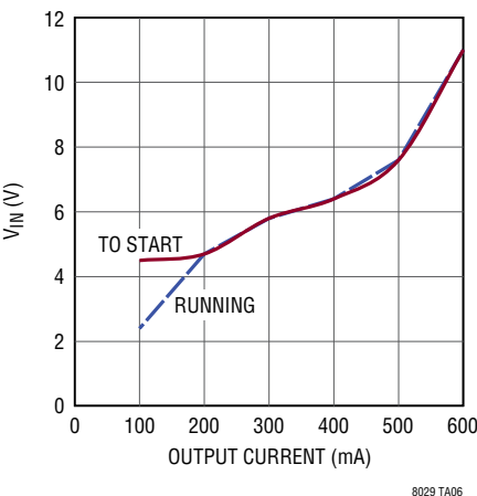
Minimum V_{IN} vs Output Current
