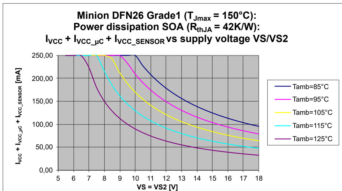
Figure 2-31. Power Dissipation and Safe Operating Area (26-pin package; Grade1): Regulator Output Currents I_{VCC} + I_{VCC\_μC} + I_{VCC\_SENSOR} versus Supply Voltage V_S at different Ambient Temperatures ( R_{thJA} = 42K/W assumed)
