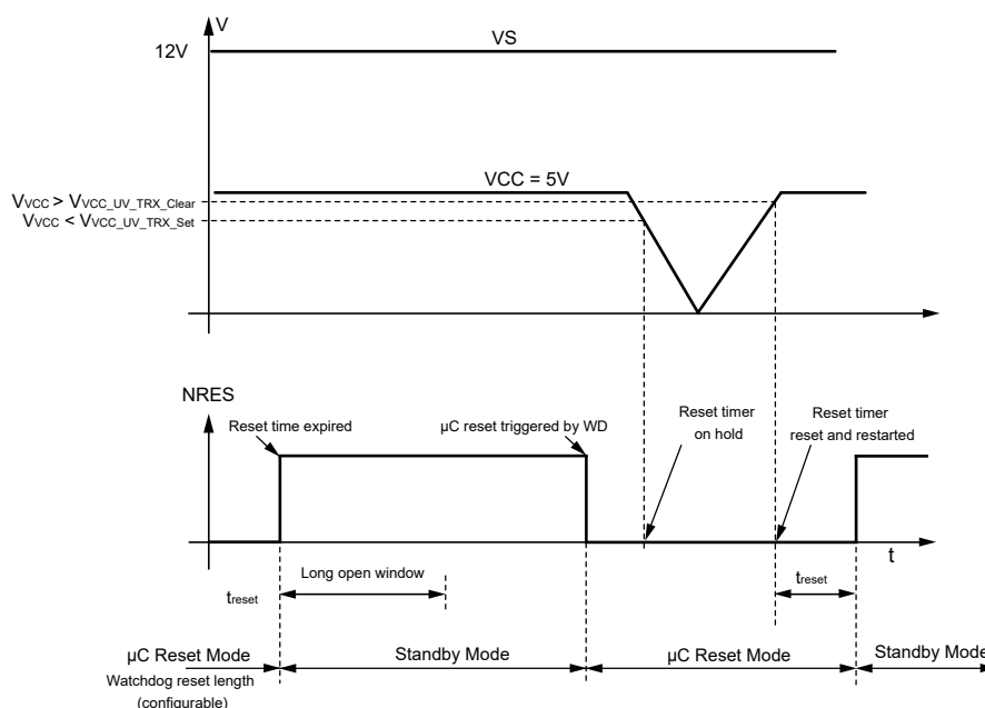
Figure 2-15. Watchdog during VCC undervoltage V_{VCC} < V_{VCC\_UV\_TRX\_Set} (RSTLVL==1)
