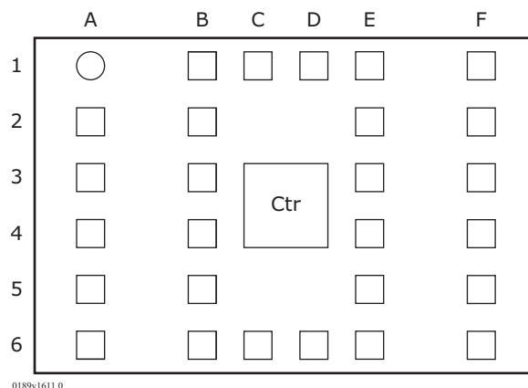
Figure 8 • ZL70123 Pad Configuration (top view)
