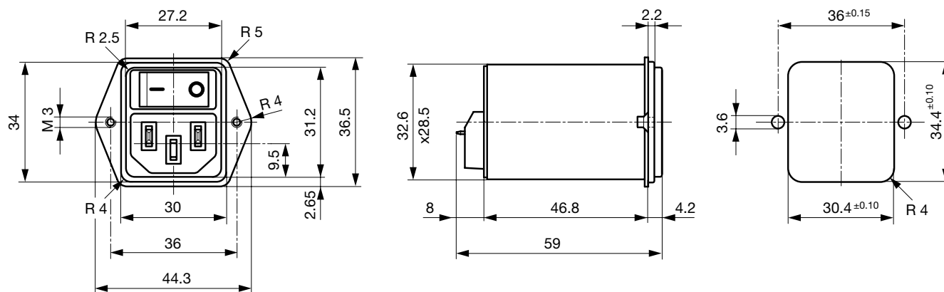
Snap-in mounting from front side (protection class II)
