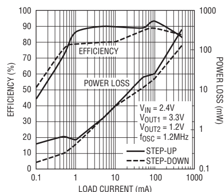
LTC3523 Efficiency and Power Loss vs Load Current
