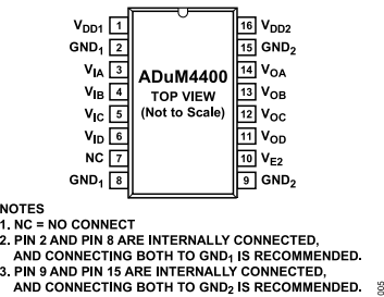
Figure 5. ADuM4400 Pin Configuration
