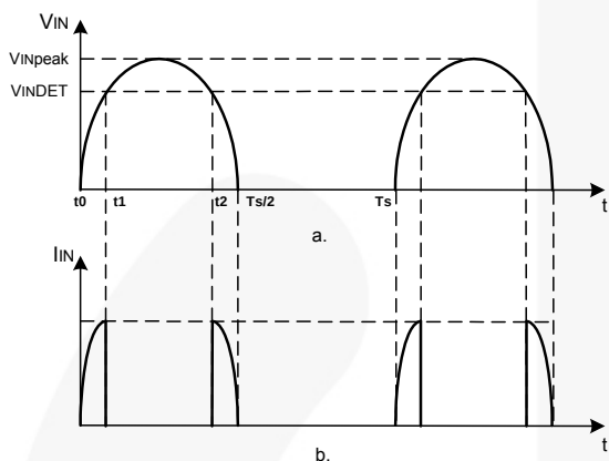
Figure 18. Typical Waveforms
