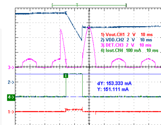
Figure 6. Current Limit
