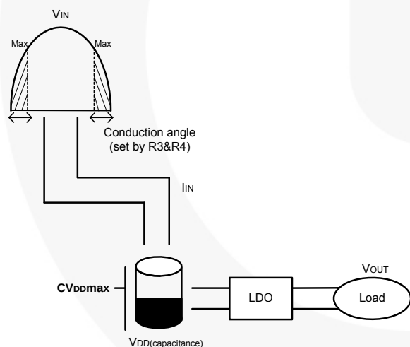
Figure 17. Operating Principle
