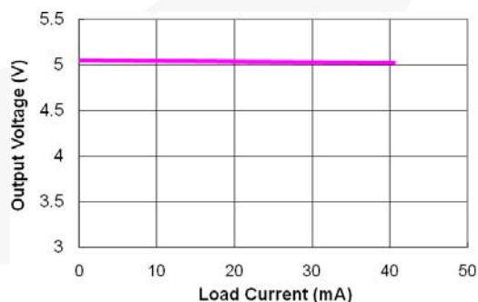
Figure 16. Output Voltage vs. Output Load
