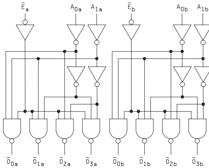
FIGURE 2. Logic diagram.
