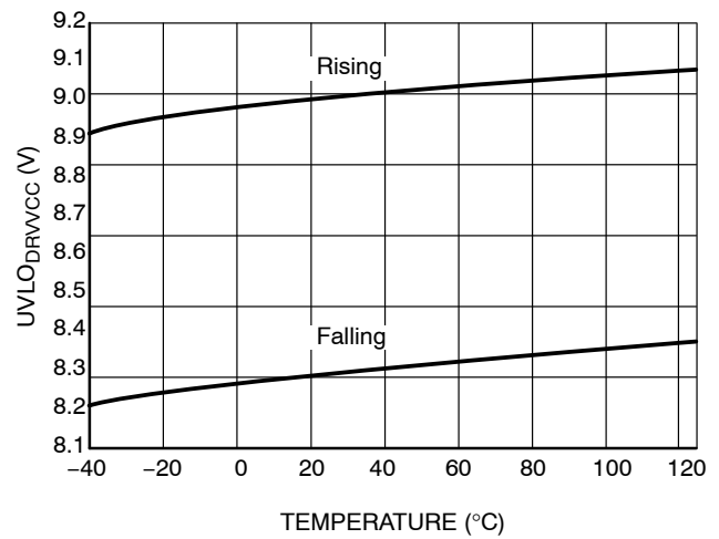
Figure 7. UVLO_{DRVCC}
