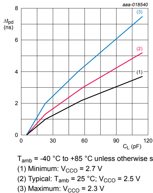
Fig. 7. Additional propagation delay versus load capacitance
