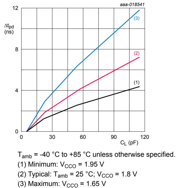
Fig. 8. Additional propagation delay versus load capacitance
