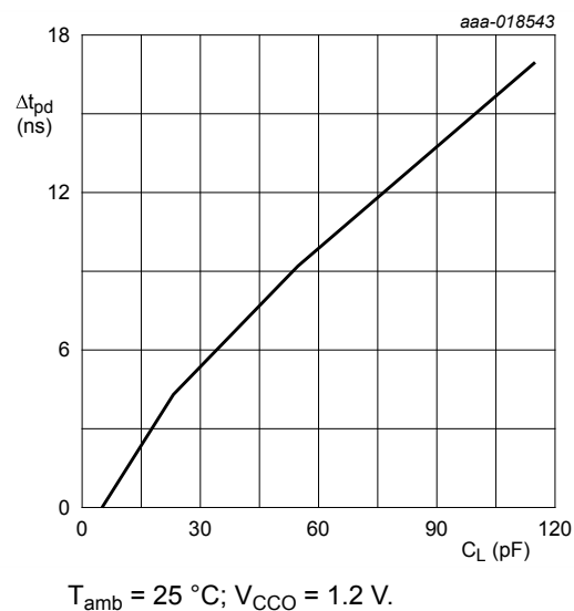
Fig. 10. Additional propagation delay versus load capacitance
