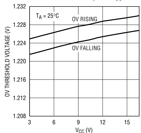
OV Threshold Voltage vs V_{CC}
