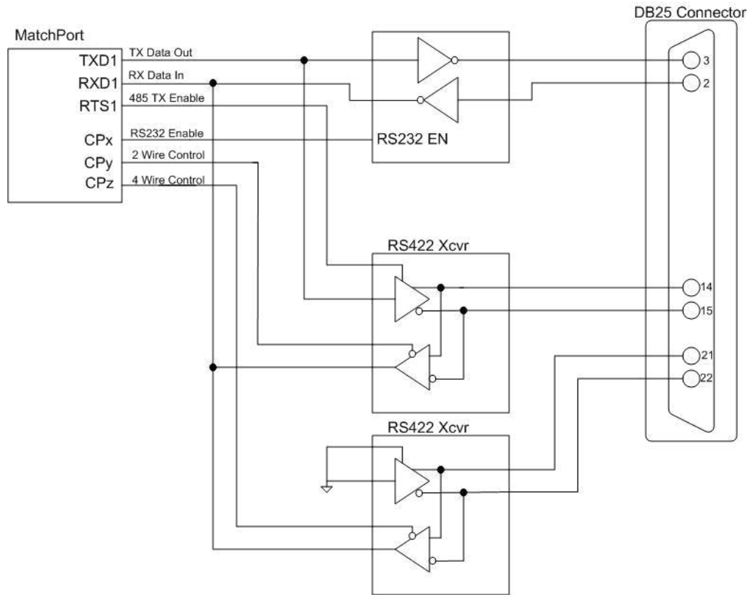
Figure 2-10. Separate RS422 Transceivers for 2-Wire and 4-Wire Setups
