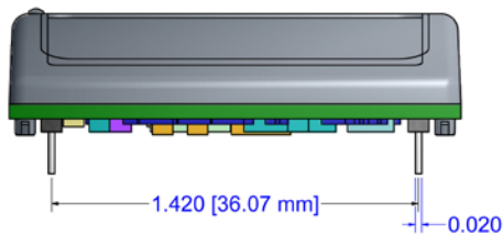
Figure 2-13. Top View
