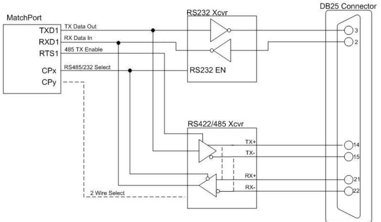
Figure 2-9. Separate RS232/422 Transceivers
