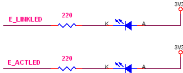
Figure 2-3. Recommended LED Connections
