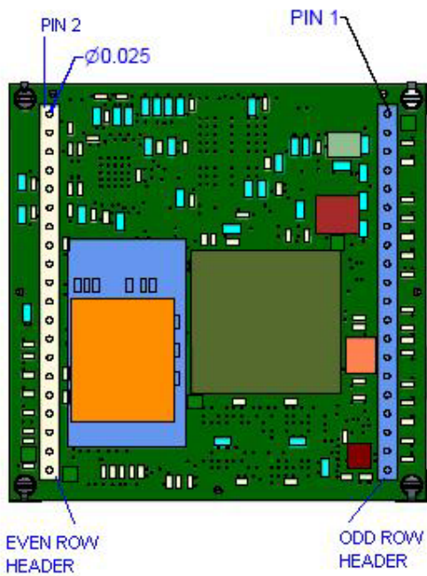
Figure 2-14. Bottom View
