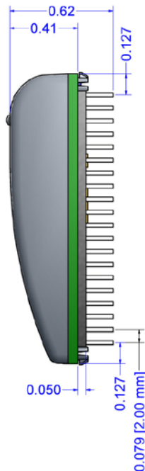
Figure 2-12. Side Views
