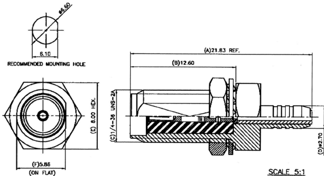
Figure 2-7. R-SMA Antenna Connector Dimensions (not to scale)
