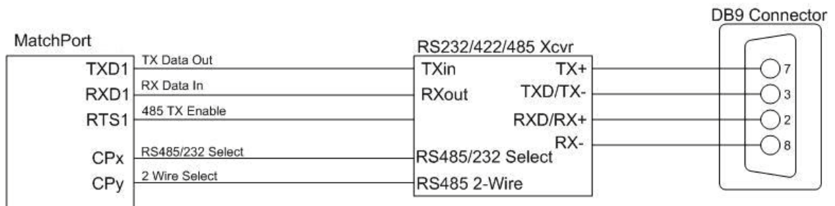
Figure 2-8. Combined RS232/422 Transceiver
