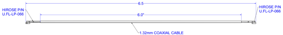
Figure 2-6. U.FL to U.FL Cable (P/N 500-181-R)
