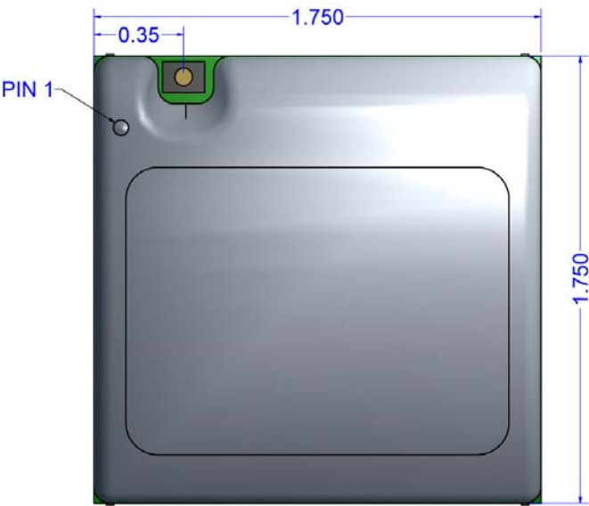
Figure 2-14. Bottom View
