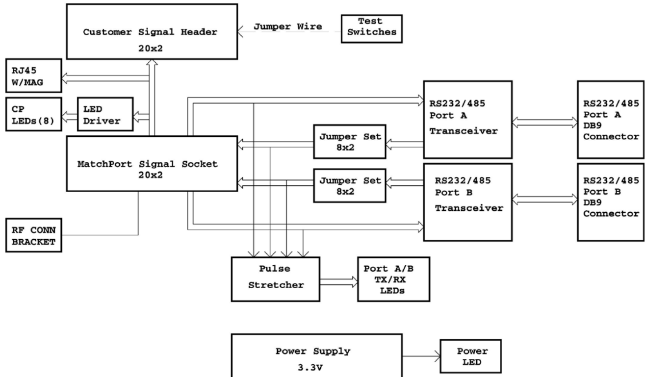
Figure 3-2. Demo Board Block Diagram
