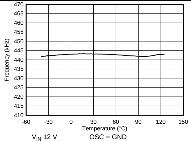
Figure 16. 440-kHz Oscillator Frequency vs Temperature
