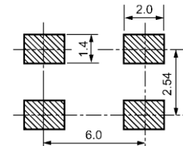
Figure 2) Suggested land pattern
