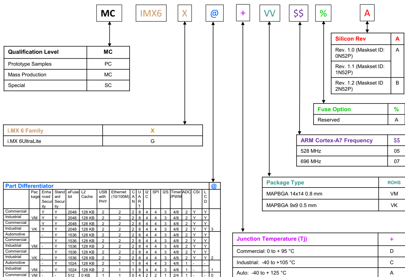
Figure 1. Part Number Nomenclature—i.MX 6UltraLite
