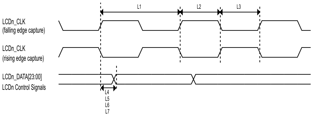
Figure 48. LCD Timing
