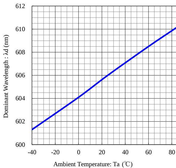
Ambient Temperature vs. Dominant Wavelength
