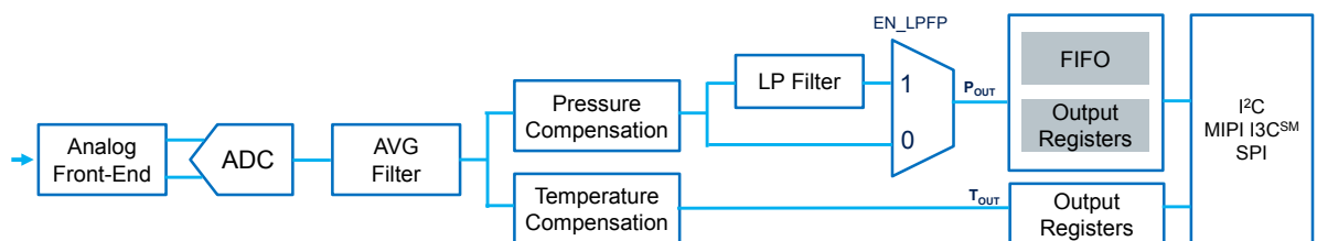
Figure 2. Digital logic
