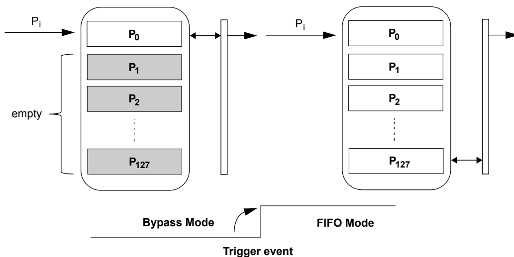
Figure 11. Bypass-to-FIFO mode
