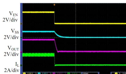
Time 200μs/div Fig. 13: Enable turn off V_{IN}=12V , V_{EN}=3.3V , V_{OUT}=3.3V , I_{OUT}=3A
