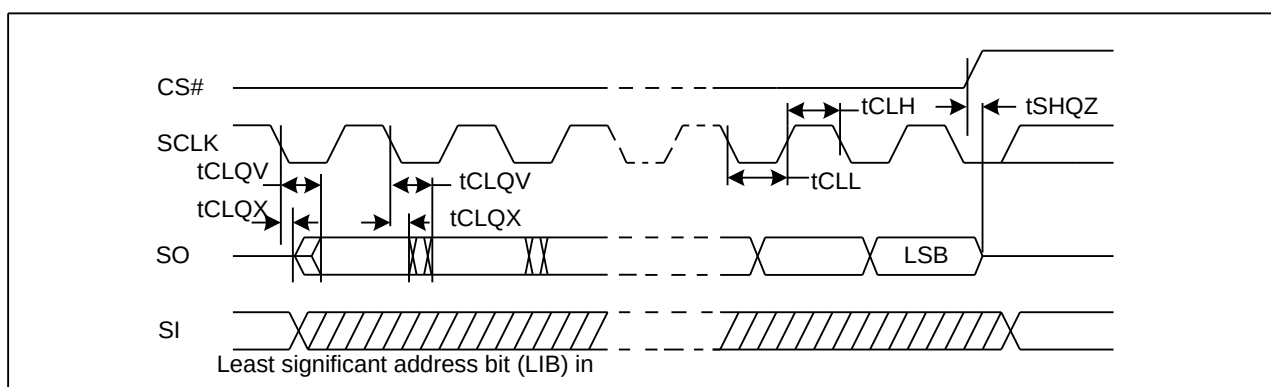
Figure 41. Output Timing
