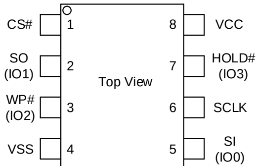
8 - LEAD VSOP/SOP
