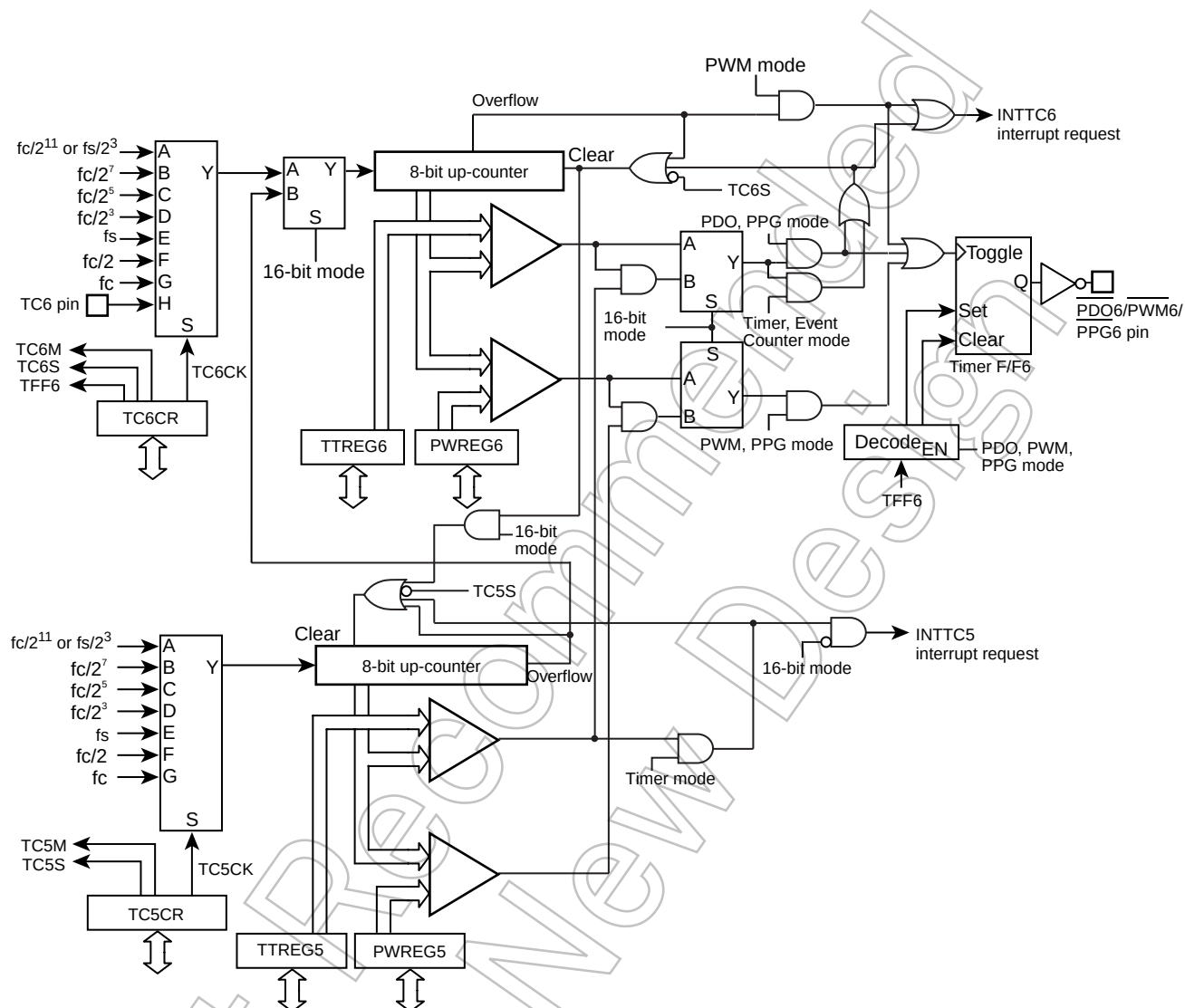
Figure 10-1 8-Bit TimerCounter 5, 6
