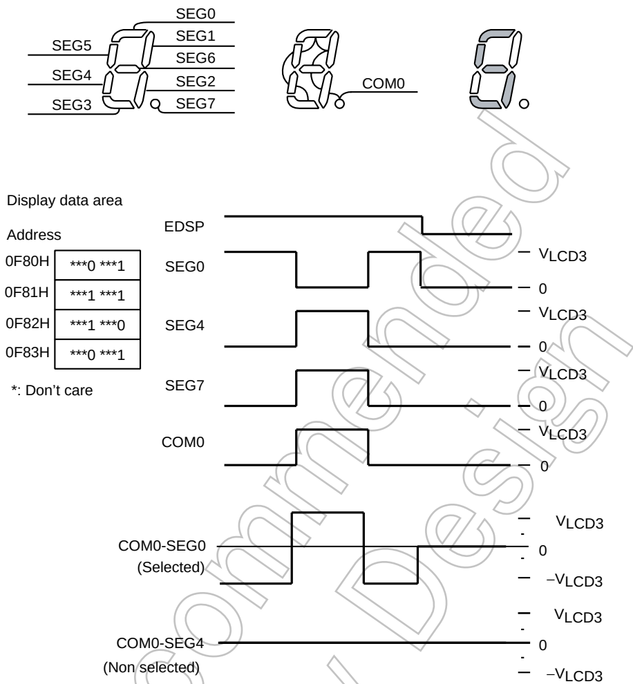
Figure 15-11 Static Drive
