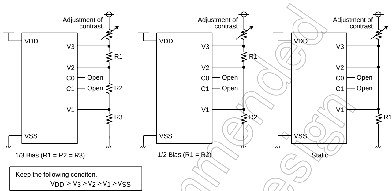
Figure 15-4 Connection Examples When Using an External Resistor Divider (LCDCCR<BRES> = "0")
