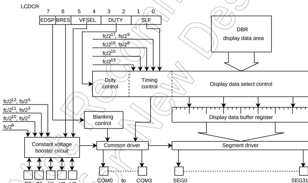
Figure 15-1 LCD Driver
