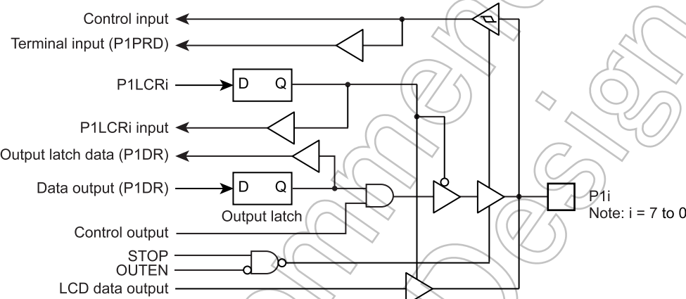
Figure 5-2 Port P1
