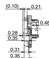
Y-Y cross section
