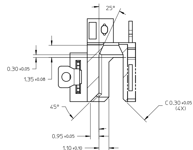
PARTIAL1 OF SECTION Z-Z
