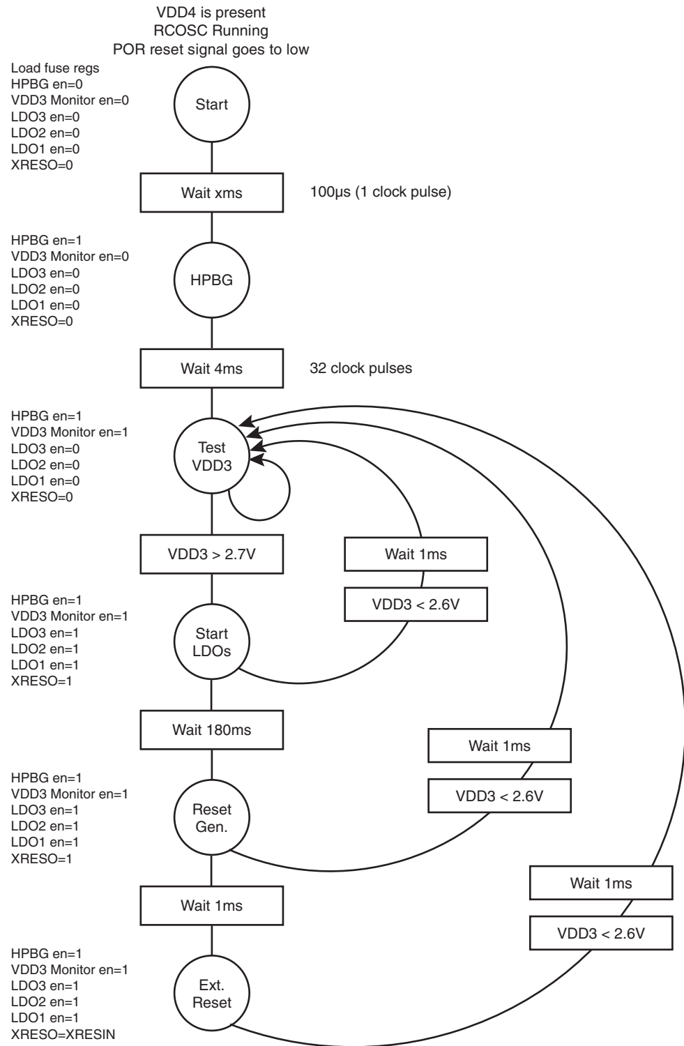
Figure 6-1. Startup Procedure
