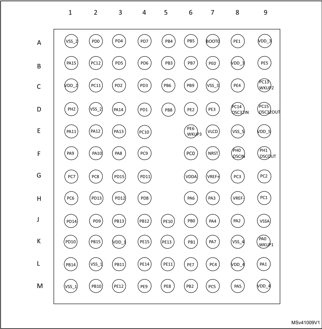
Figure 4. STM32L151VD-X WLCSP104 ballout
