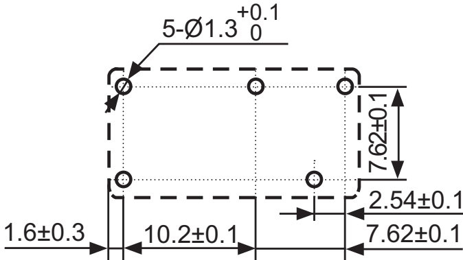
Recommended PCB Layout Bottom View
