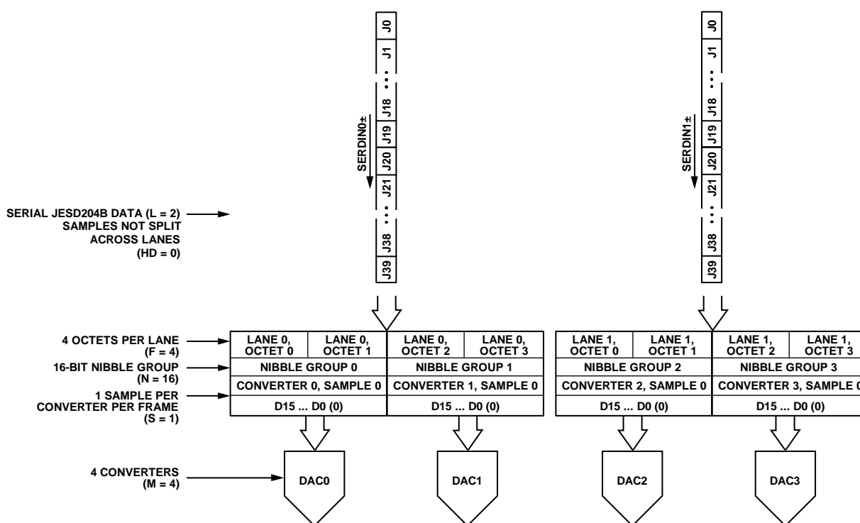
Figure 62. JESD204B Mode 3 Data Deframing
