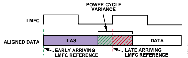
Figure 51. Link Delay > LMFC Period Example
