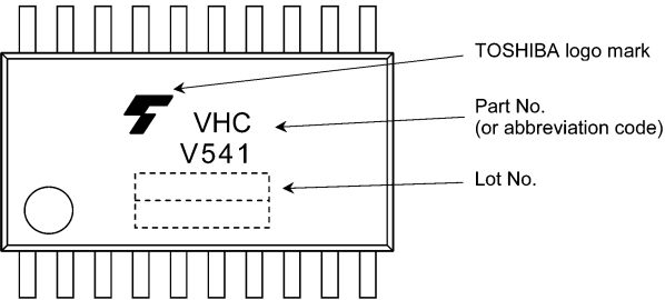
74VHCV541FT
