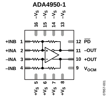
Figure 1. ADA4950-1
