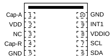
Pin Connections
