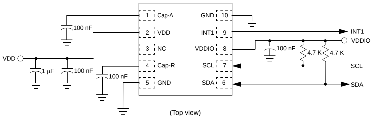
Figure 3. Electrical connection
