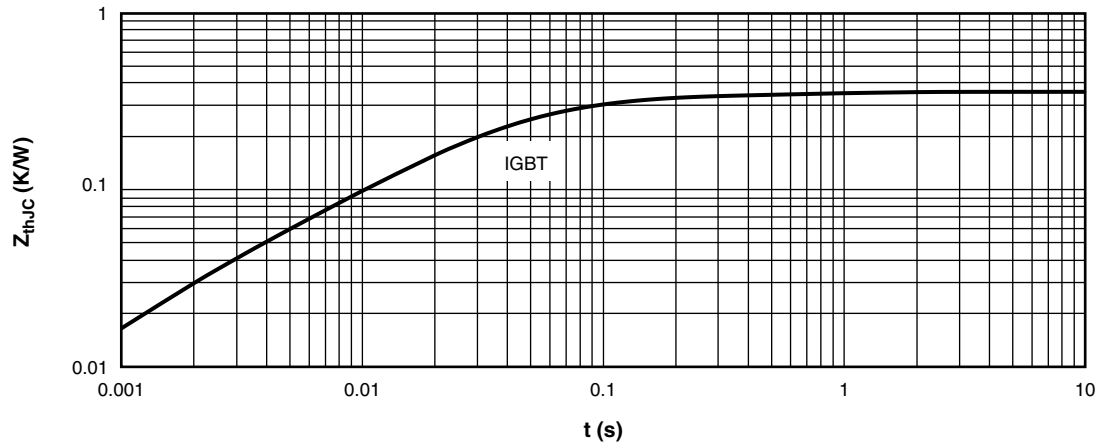
Fig. 6 - IGBT Transient Thermal Impedance
