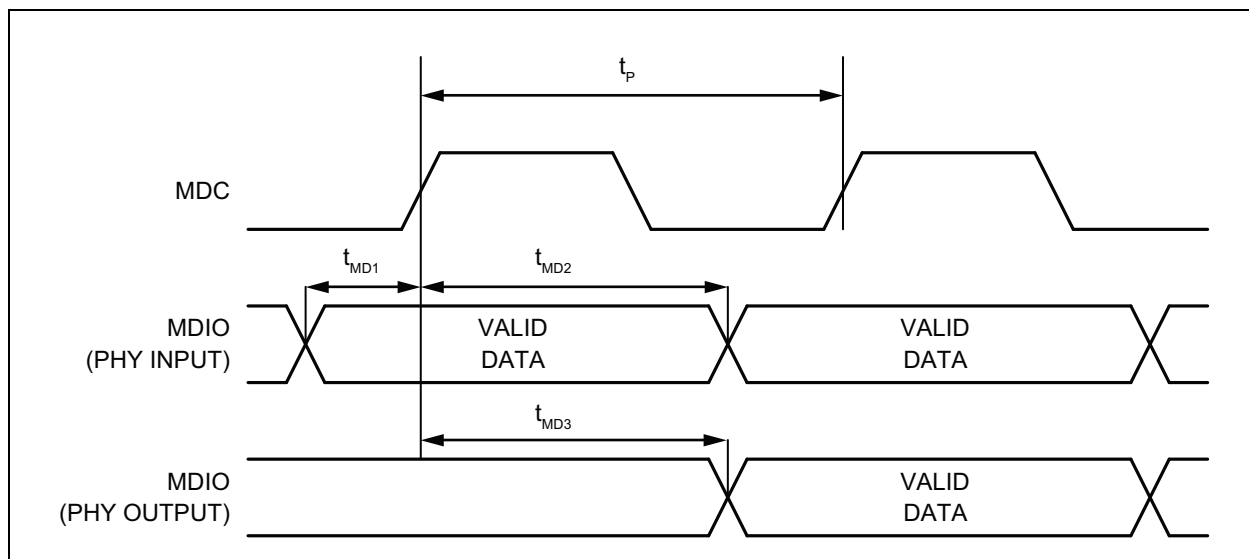
FIGURE 7-10: MDC/MDIO TIMING
