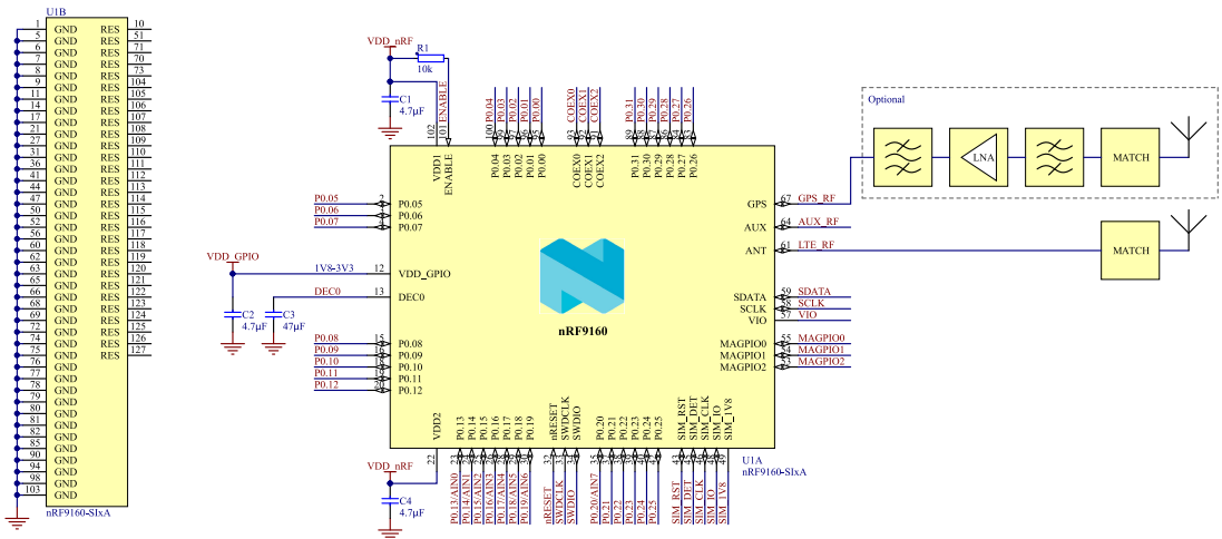
Figure 119: Schematic SlxA with antenna details
