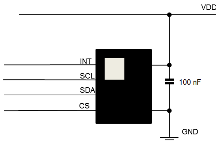
Figure 15. Application schematic with SPI connection
