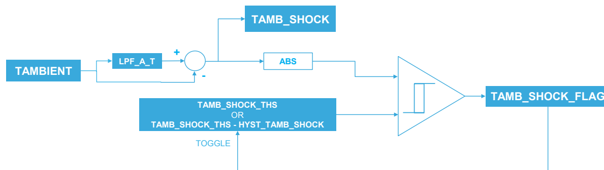
Figure 13. Block diagram of ambient temperature shock detection algorithm
