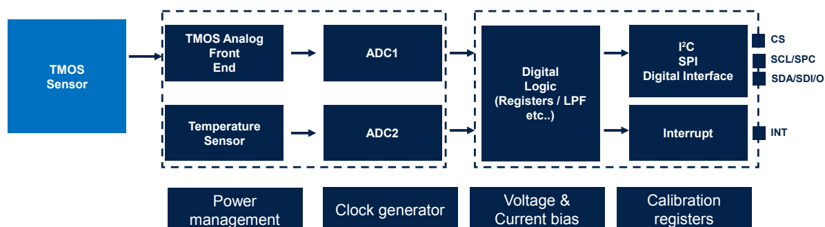
Figure 1. Block diagram
