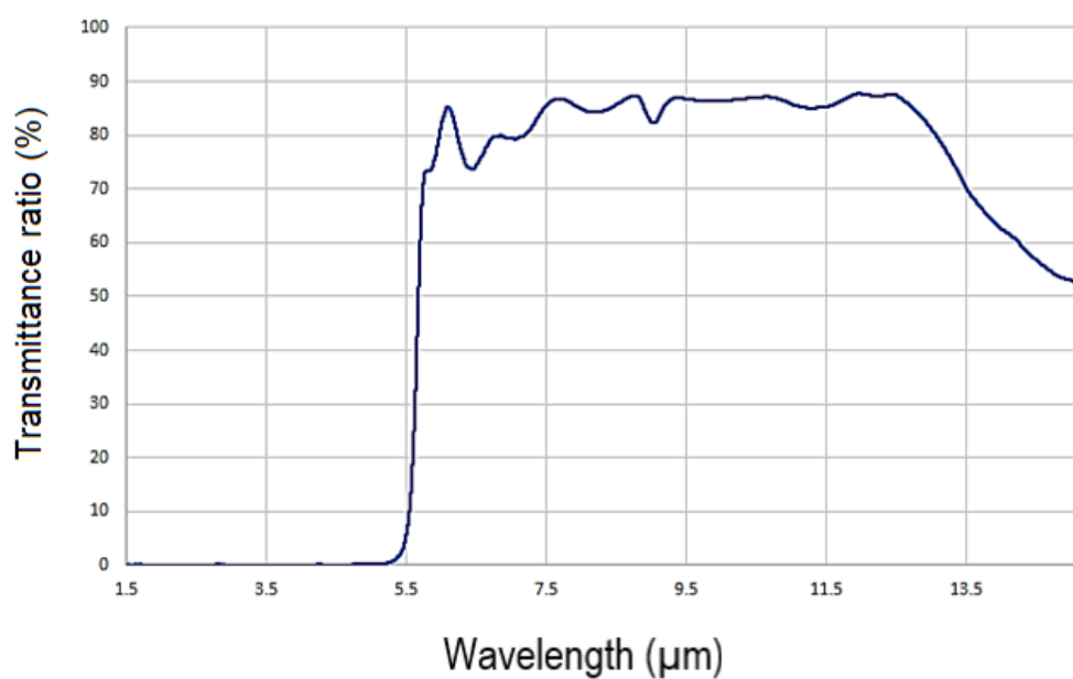
Figure 6. Filter transmittance typical curve
