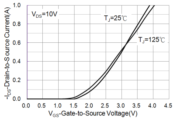
Fig.2 Transfer Characteristics
