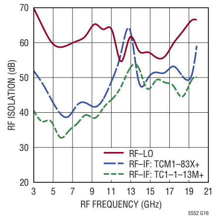
RF Isolation
