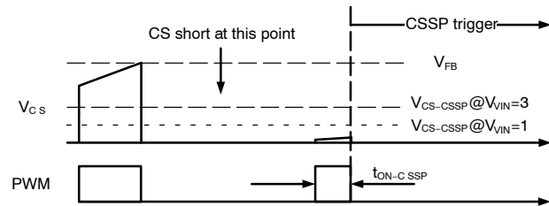
Figure 42. CSSP Waveform
