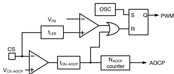
Figure 40. AOCP Logic
