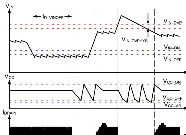
Figure 43. Brown-in/out & Line-OVP
