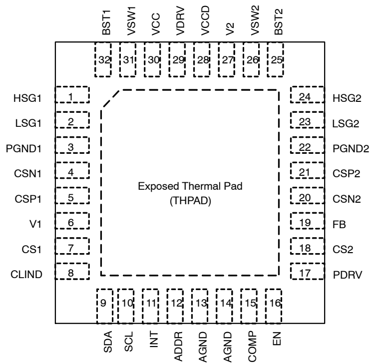
Figure 2. Pinout
