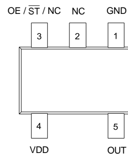
Figure 1. Pin Assignments
