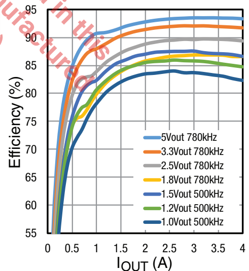
Figure 2: Efficiency 12VIN
