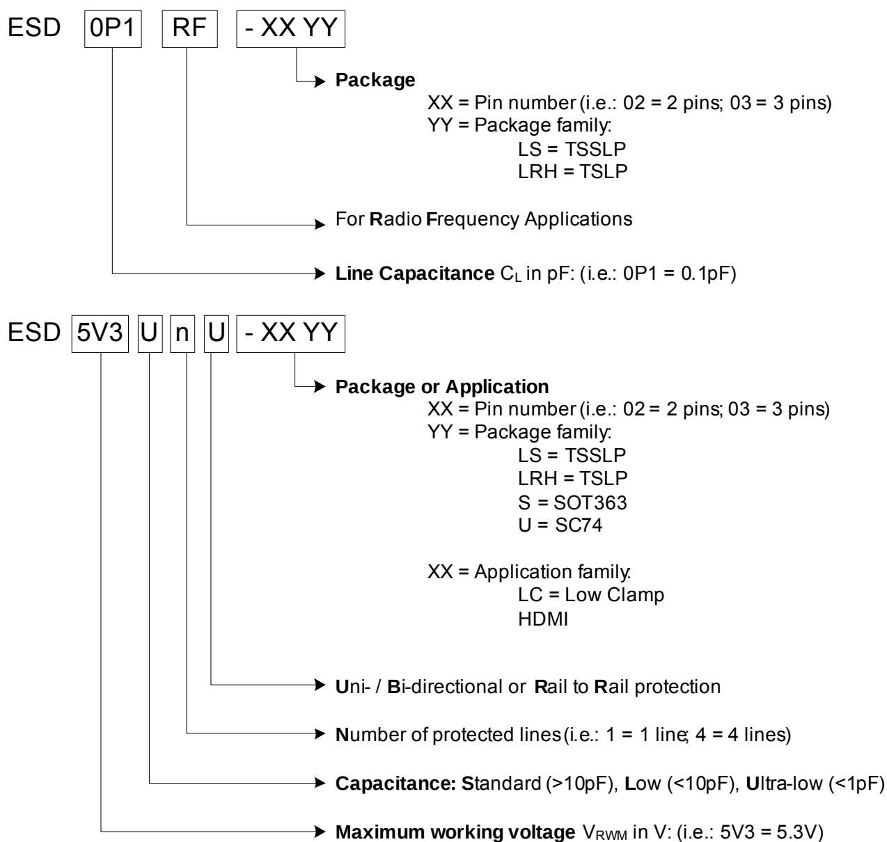
Figure 11 Ordering information scheme
