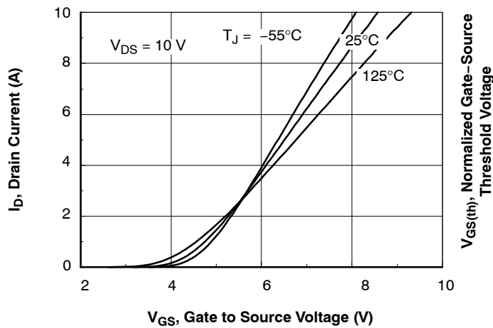
Figure 5. Transfer Characteristics
