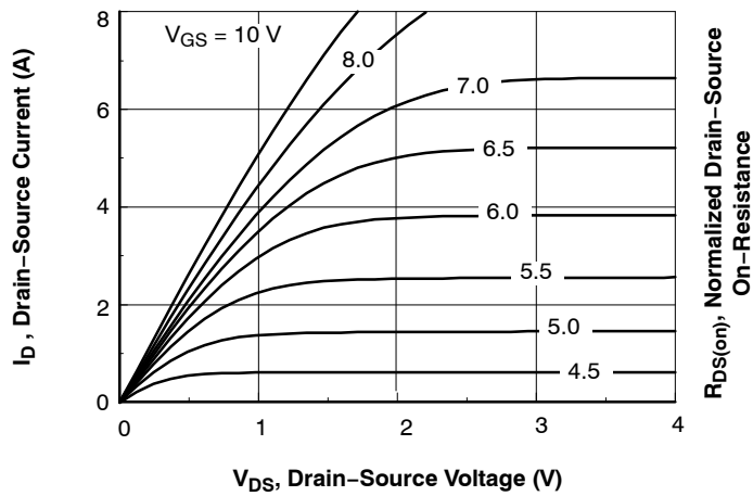
Figure 1. On-Region Characteristics
