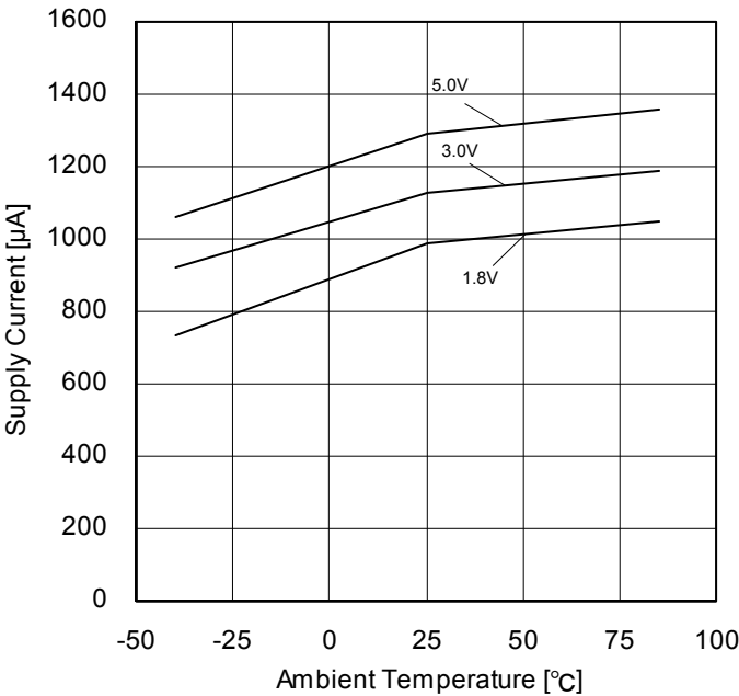
Figure 56. Supply Current vs Ambient Temperature
