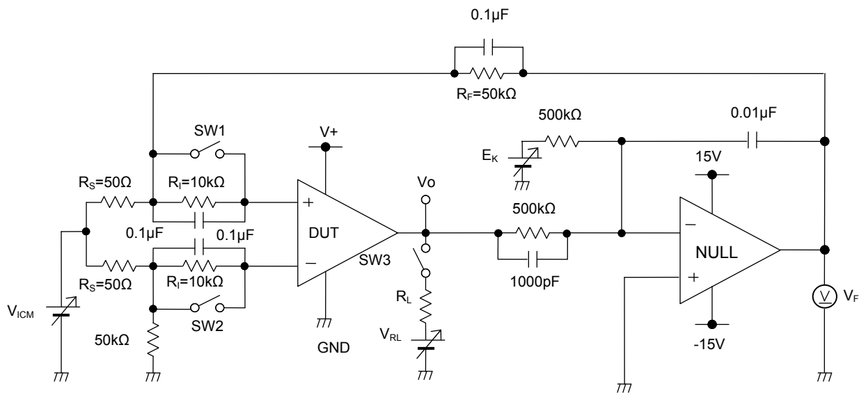
Figure 81. Test Circuit 1
