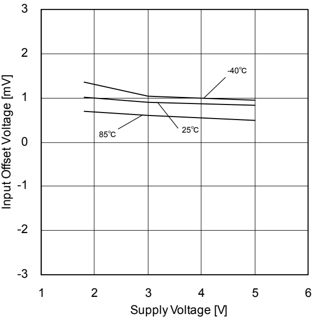
Figure 12. Input Offset Voltage vs Supply Voltage
