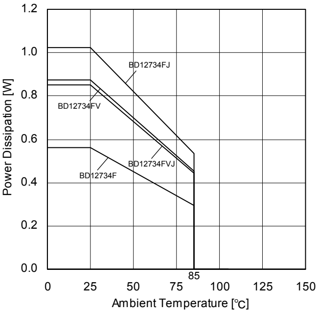
Figure 54. Power Dissipation vs Ambient Temperature (Derating Curve)
