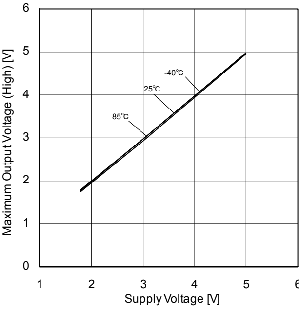
Figure 57. Maximum Output Voltage (High) vs Supply Voltage ( R_L=20k\Omega )
