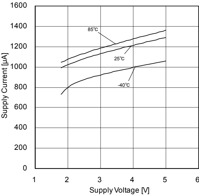
Figure 55. Supply Current vs Supply Voltage
