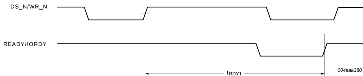
Fig 24. ISP1583 ready signal timing
