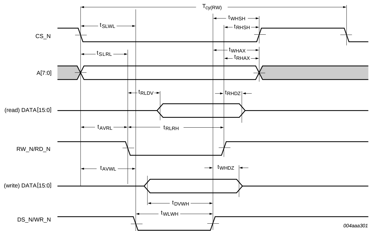
Fig 21. ISP1583 register access timing: separate address and data buses (8051 mode)
