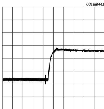
Fig 9. Oscilloscope reading: with resistor and capacitor in the network
