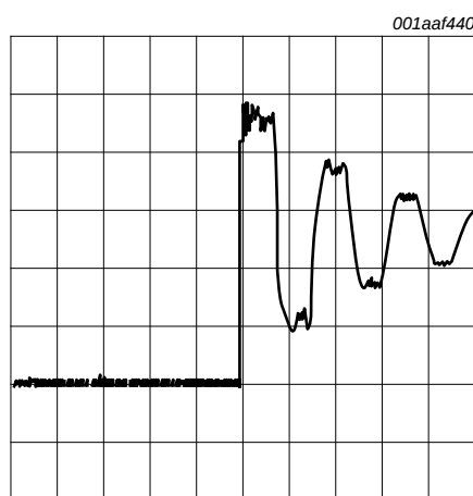
Fig 8. Oscilloscope reading: no resistor and capacitor in the network
