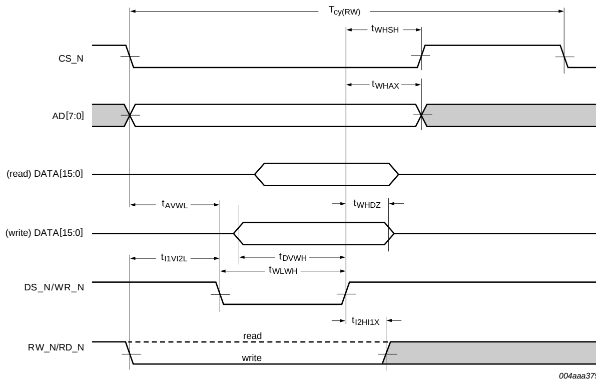
Fig 23. ISP1583 register access timing: separate address and data buses (Freescale mode)
